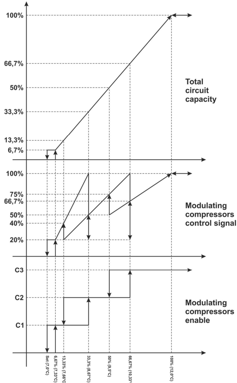
3 modulating compressors 33,3% capacity each Min value = 20% (6,7% total capacity) Set = 7°C, PB = 5°C
